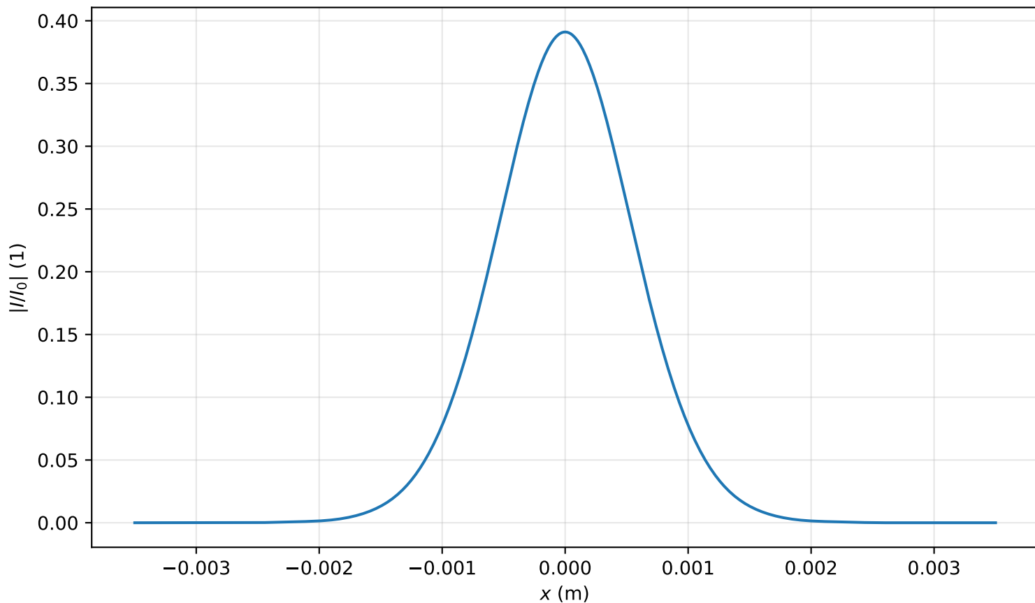
Intensity profile I(x, y = 0, z = 3.184m)/I_0 , P_{in}=0.3P_{cr} , artificial time
